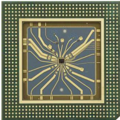
Every Z-Series oscilloscope has Keysight’s custom InP fast edge.
