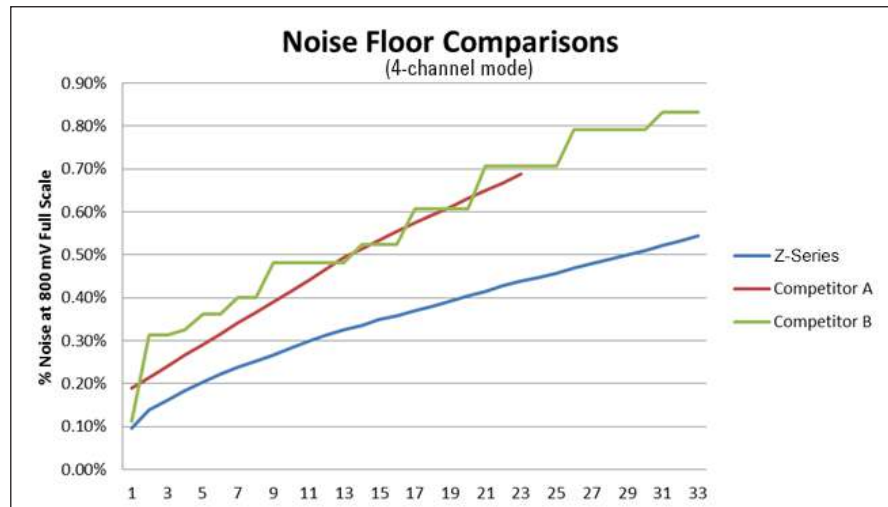
The Z-Series features the industry's lowest noise floor.
