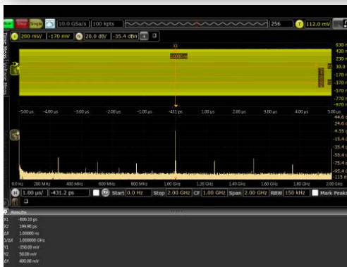
Easy-to-use FFTs
