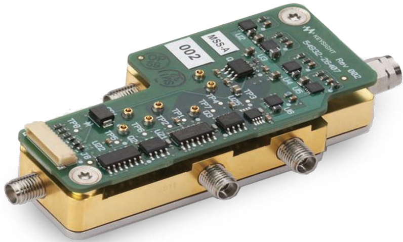
RealEdge technology blocks enable 63-GHz real-time bandwidth.
